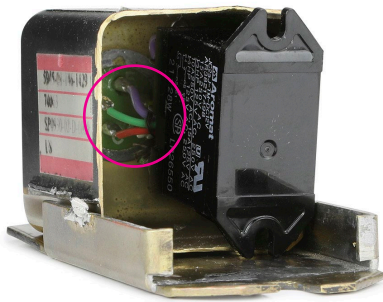
Original Ignition Relay Mechanical relay having under-rated voltage and power for intended service with inferior, appliance grade construction
